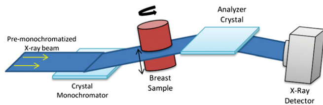
Fig. 1. Schematic diagram of the phase contrast X-ray imaging set-up. A collimated X-ray beam with energy of 60 keV was monochromatized by a double Si (111) crystal system and an additional single Si (333) crystal. The breast cancer sample was mounted on a rotary stage and positioned in the X-ray beam. The refracted and scattered X-rays by the sample were analyzed by a Si (333) analyzer crystal. The analyzer crystal was rotated according to the incoming X-ray beam and set at an angle close to the Bragg diffraction condition. After each rotation, the sample was vertically displaced relative to the X-ray beam, allowing a different region to be imaged. A fast-readout and low-noise charge-coupled device (CCD) camera with 2,048 \times 2,048 pixels was used to measure the phase contrast X-ray images.
